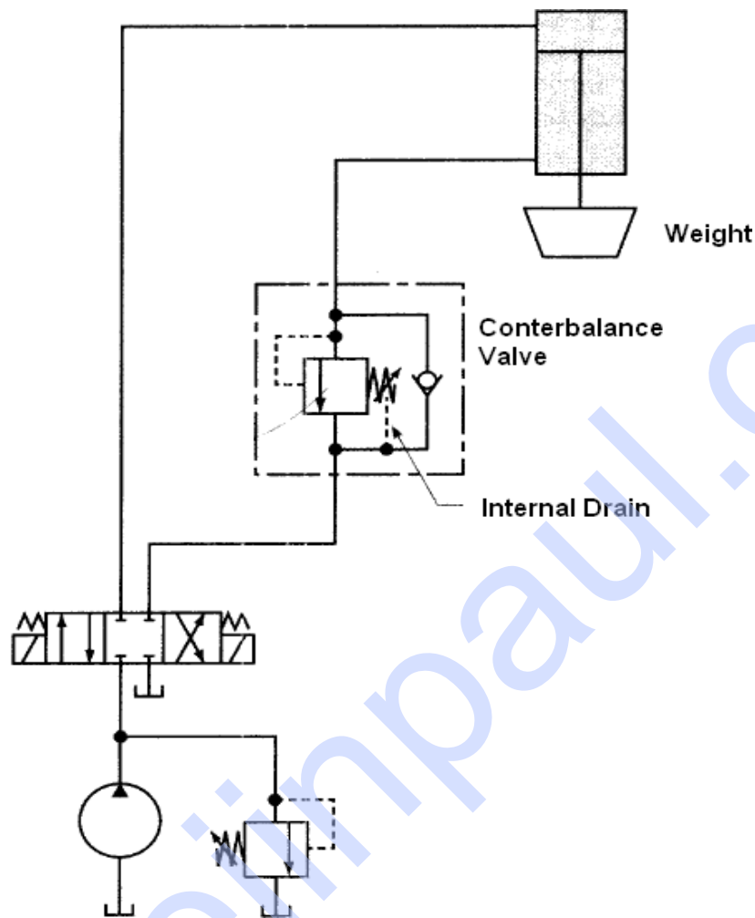
Counterbalance Circuit
