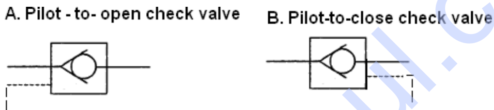
Symbols for Pilot Operated Check Valve
