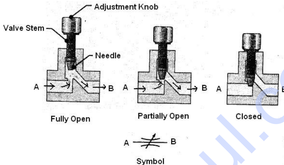
Needle Valve
